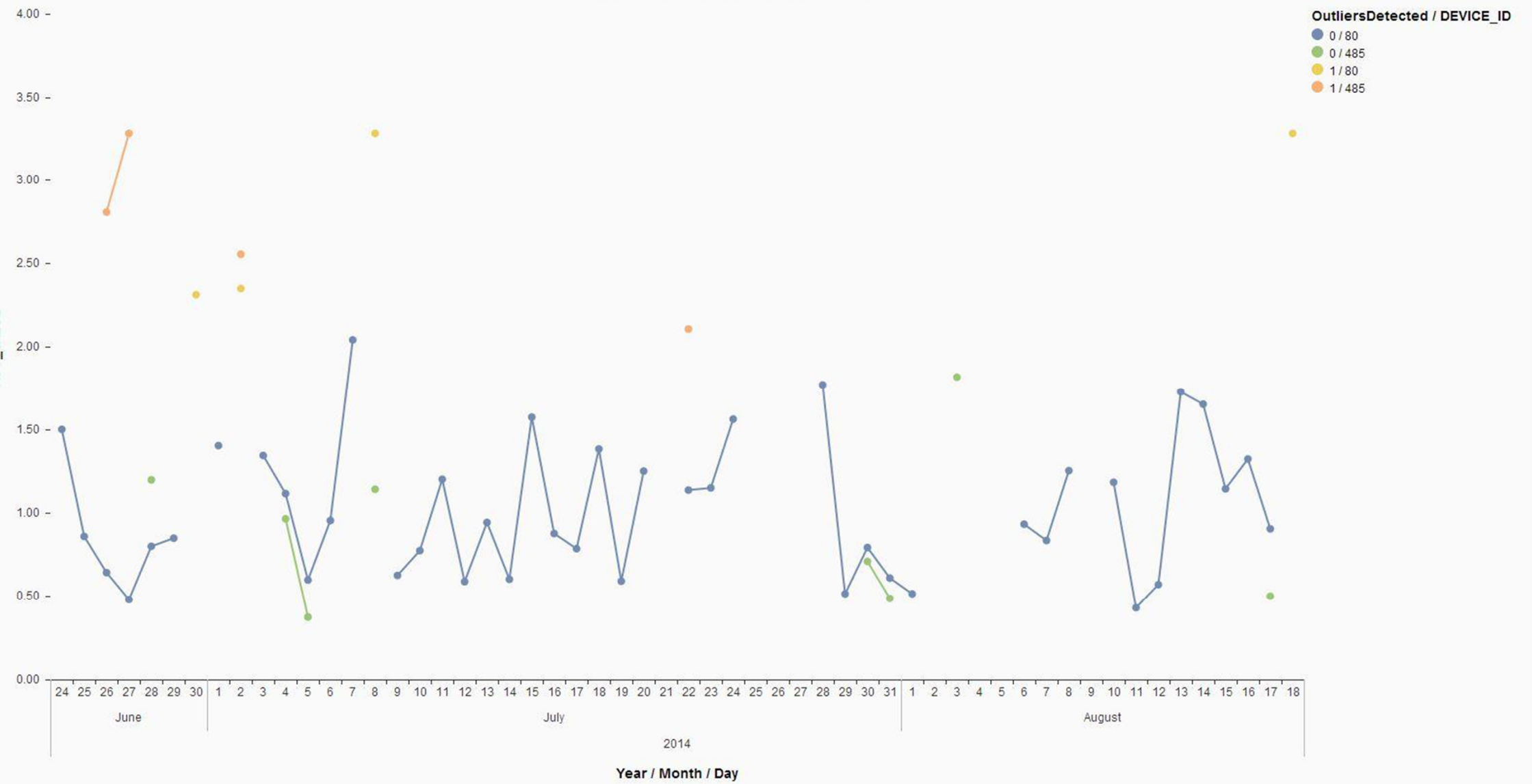
AVG_VALUE by OutliersDetected, DEVICE_ID and Day
